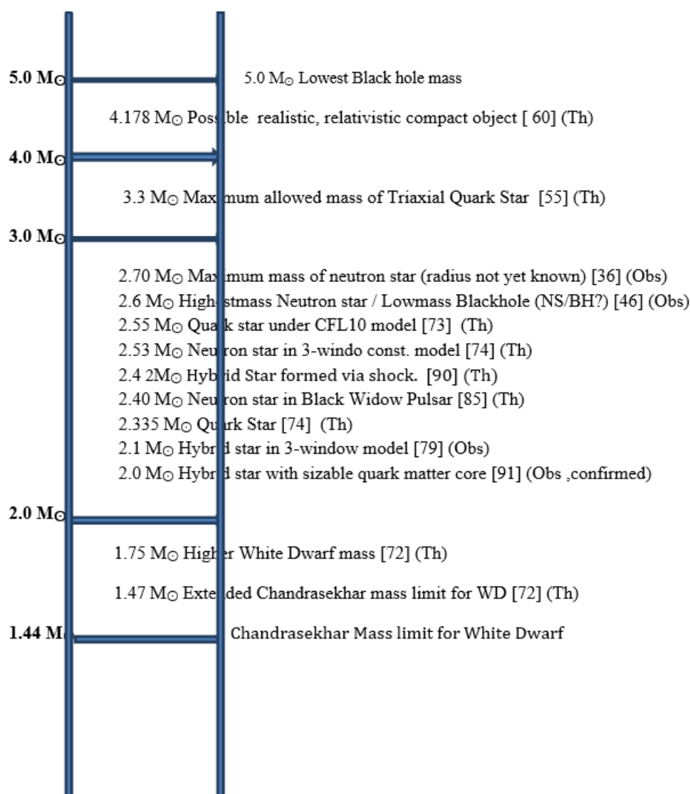
Fig. 1. Mass Gap Ladder for different compact objects with their maximum masses (not scaled)
