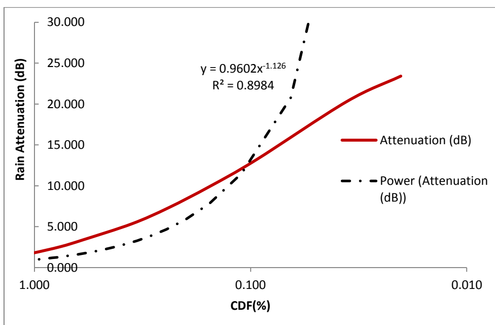
Fig. 4. Relationship between CDF and rain attenuation for August 2019
