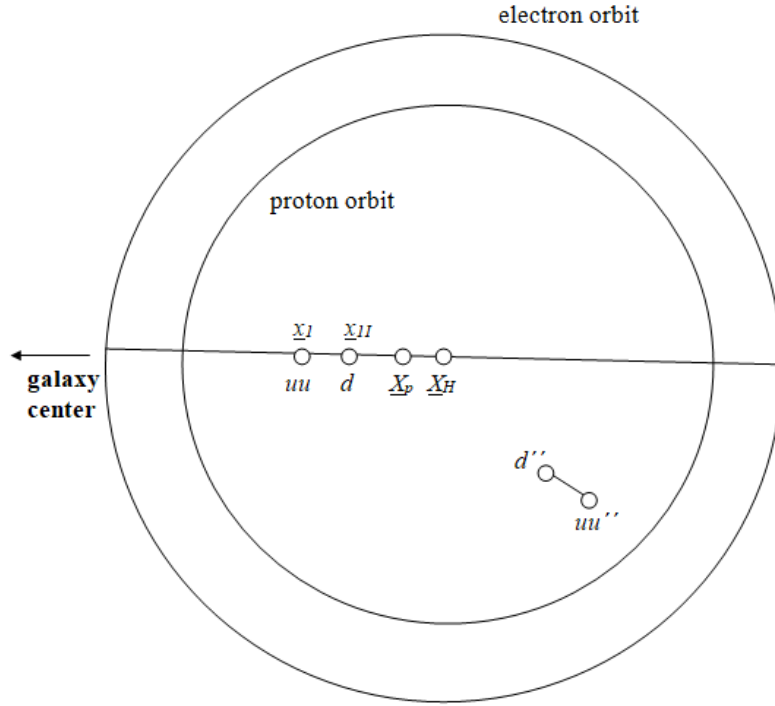
Fig. 2. Schematic structure of the test hydrogen atom in Figure 1 before and after a collision with another hydrogen atom in interstellar medium. The uu - d quarks before the collision have been moved to the positions denoted by uu'' - d''
