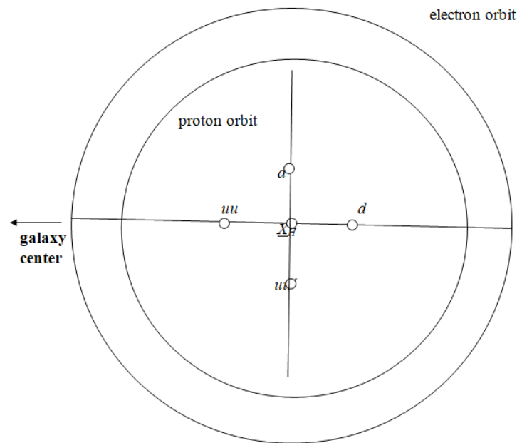
Fig. 1. Schematic structure of a free, test hydrogen atom in SSI. The large electron orbit has been scaled down to fit inside this figure. X_H denotes the coordinate of the center of this test atom. It is also the center X_e of the electron charge cloud having a radius of 0.53\text{\AA} (Bohr radius a_0 , outer circle) as well as the center X_p of the proton charge cloud having a radius of 28.8\text{ fm} (proton Bohr radius a_{0p} , inner circle). The small distance r = |x| between the uu' (or uu ) diquark and the d' (or d ) quark has been scaled up for illustration. In the absence of gravitational field, x can form any angle with the horizontal axis. Here, the angles 0^\circ for uu - d and 270^\circ for uu' - d' have been chosen for illustration. When a gravitational field is present, as is indicated by the left arrow towards a galaxy center, the vector x will align itself along direction of this field. The quarks will now lie on the horizontal axis with heavier uu diquark closer to the galaxy center
