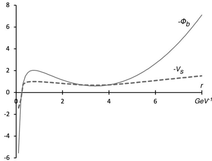
Fig. A1. Strong interaction potential \Phi_b in units of \text{GeV}^3 in the equations of motion for neutron (A19) specified by (A24) with d_{b2} = -0.3202 \text{ GeV}^5 , d_{b1} = 2.272 \text{ GeV}^4 , d_{b0} = -0.4.922 \text{ GeV}^3 , and d_{b0} = 1.024 \text{ GeV}^5 [4 Table 11.1]. The u - d strong interaction potential -V_s in units of \text{GeV} is inferred from (A22). The unit of r is \text{GeV}^{-1} = 1.24 \text{ fm}
