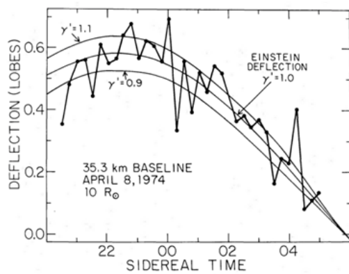
Fig. 19. Measurement data at 10 solar radii
