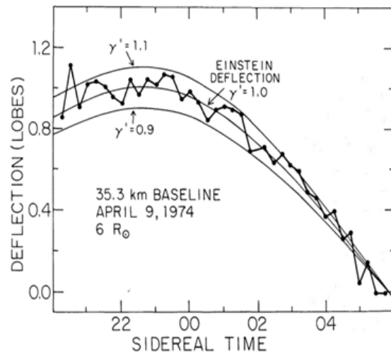
Fig. 18. Measurement data at 6 solar radii
