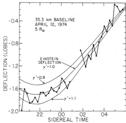
Fig. 17. Measurement data at 3 solar radii
