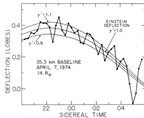
Fig. 20. Measurement data at 16 solar radii
