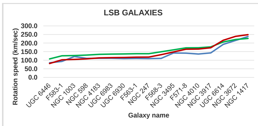
Fig. 3. Galactic rotation speeds of LSB galaxies
