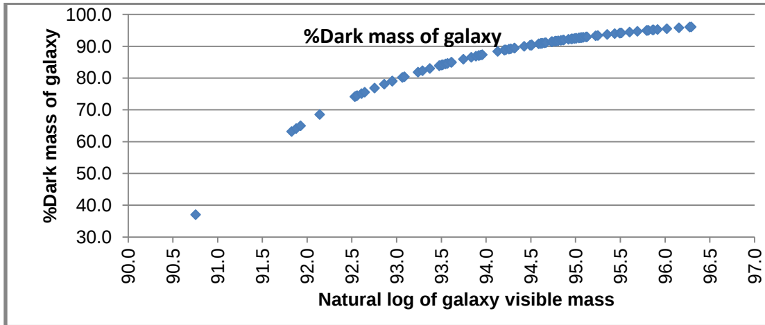
Fig. 1. Estimated galactic dark mass parentage
