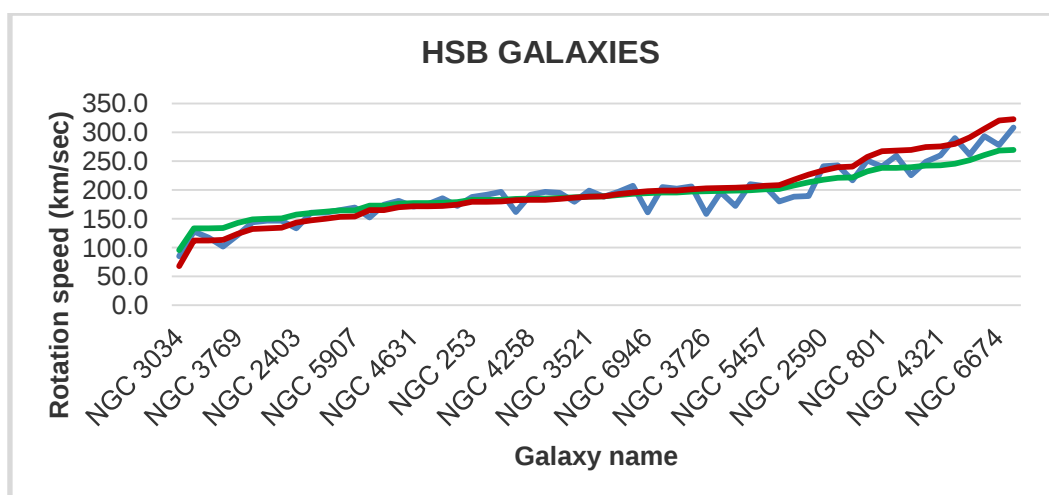
Fig. 4. Galactic rotation speeds of HSB galaxies
