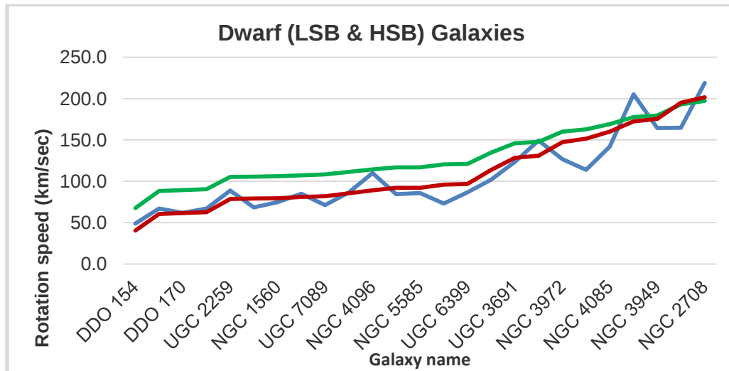
Fig. 2. Galactic rotation speeds of Dwarf galaxies
