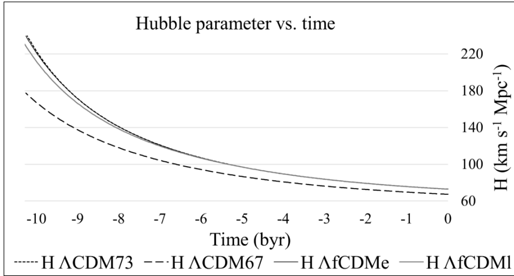
Fig. 2. Hubble parameter H vs. time for the various universes
